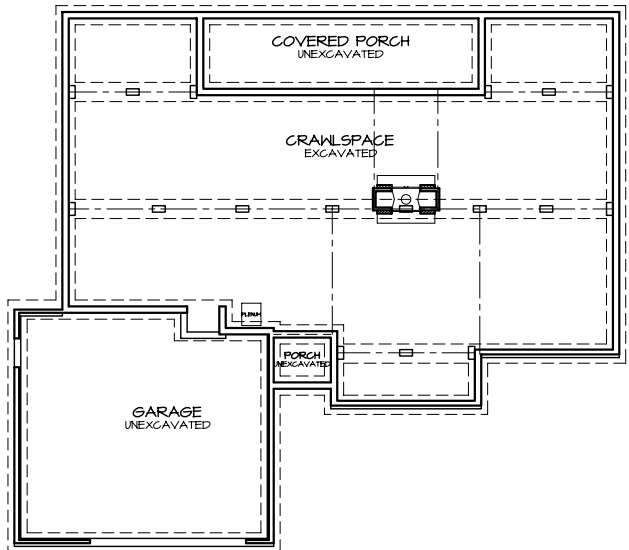
1 FOUNDATION PLAN A-3
